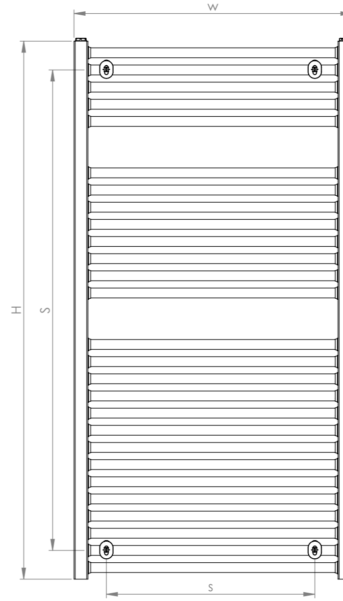
Assembly Axis
